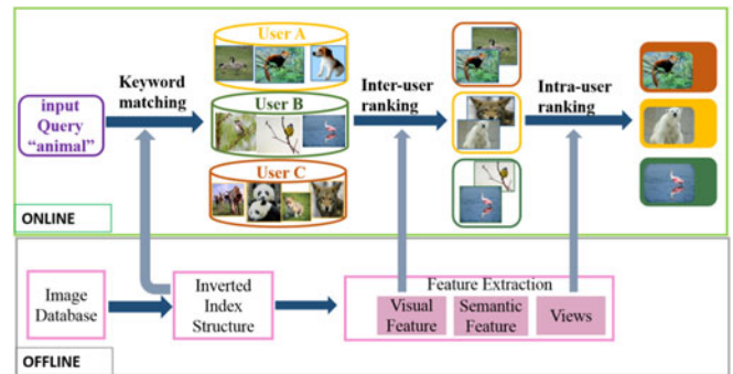
Fig. 1. System framework of tag-based image retrieval with social re-ranking.
